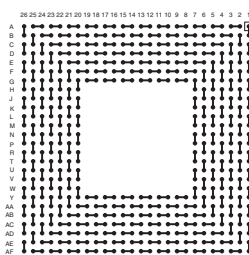
LBGA532T.8-DC266
