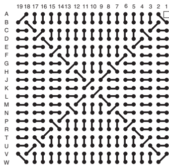
LPGA357T1.27-DC73
