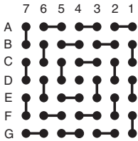
BGA49T.8-DC077
