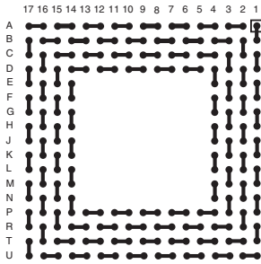
BGA208T1.27-DC170
