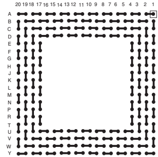
BGA256T1.27-DC200
