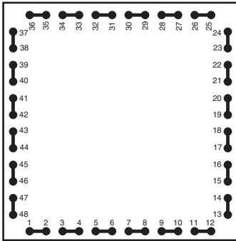
FC48 (PB18 - 250x250)
