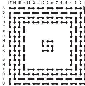
BGA217T1.27-DC172
