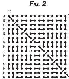
BGA225T1.5-DC15
