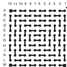
LBGA144T.8-DC128
