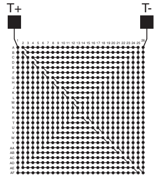
BGA676 AFTER ASSEMBLY
