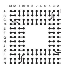
LBGA144T.8-DC134
