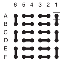
BGA36T.8-DC069
