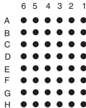
BGA48T.75-6x8
