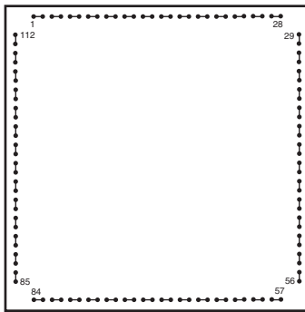
FC112 (PB06 - 200x200)
