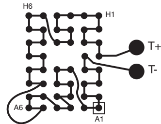
AFTER MOUNTING TO TEST BOARD
