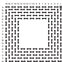
LBGA280T.8-DC195
