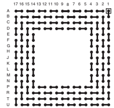
LBGA208T.8-DC170
