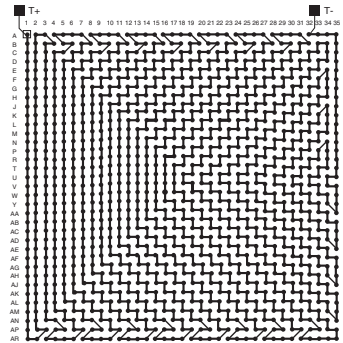
LBGA1225-DC359 After Mounting
