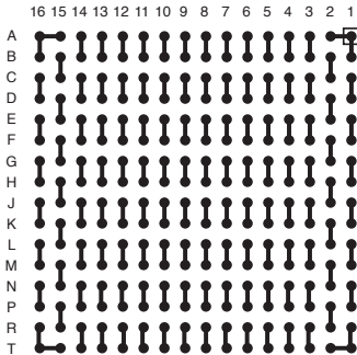
LPGA256T1.27-DC61
