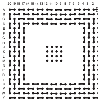
BGA272T1.27-DC202
