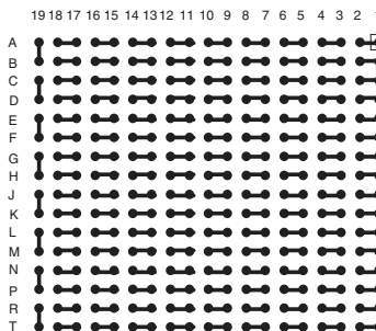
CBGA304T1.27-DC63
