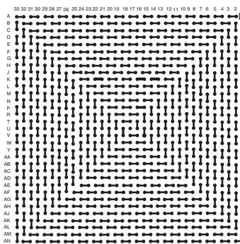
CBGA1089T1.27-DC339
