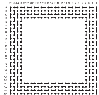
BGA352T1.27-DC70
